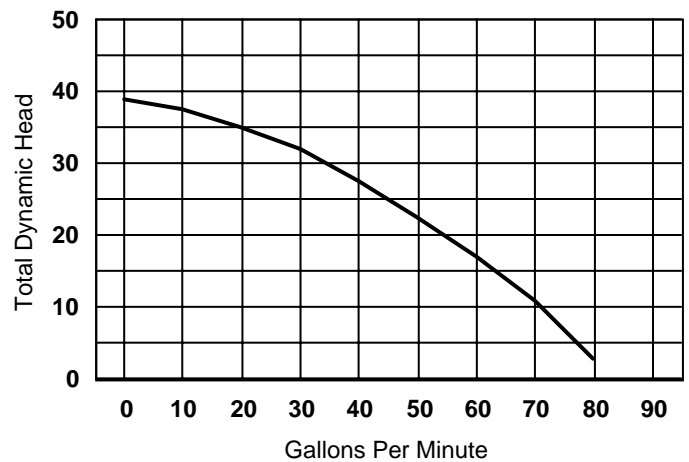
Piranha Model P-75-SS .75 hp 115v 1 ph
