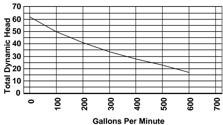
Piranha Solids Handling Pump Model PLS 500
