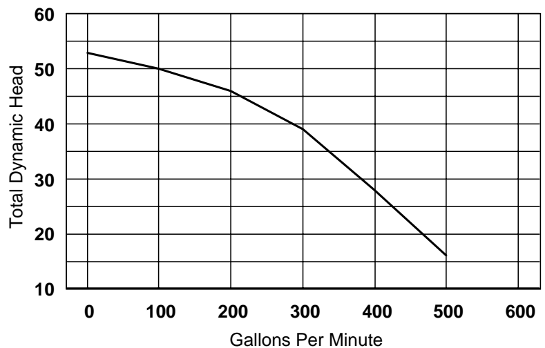
Piranha Agitator Pump Model PS750A
