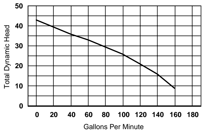
Piranha Model PSS-200 2 hp 230v,460v
