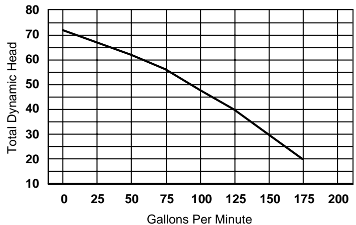
Piranha pump model PSS-300 3 hp, 230v/460v, 3 phase
